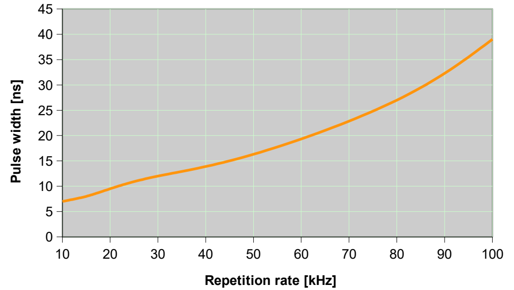
Sol 20W 532nm: Pulse Width
