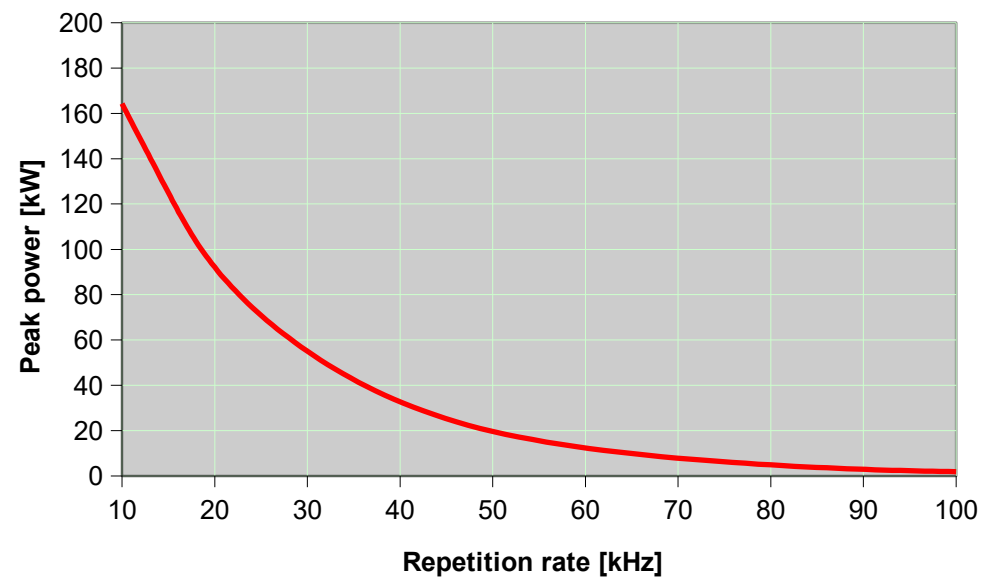
Sol 20W 532nm: Peak Power
