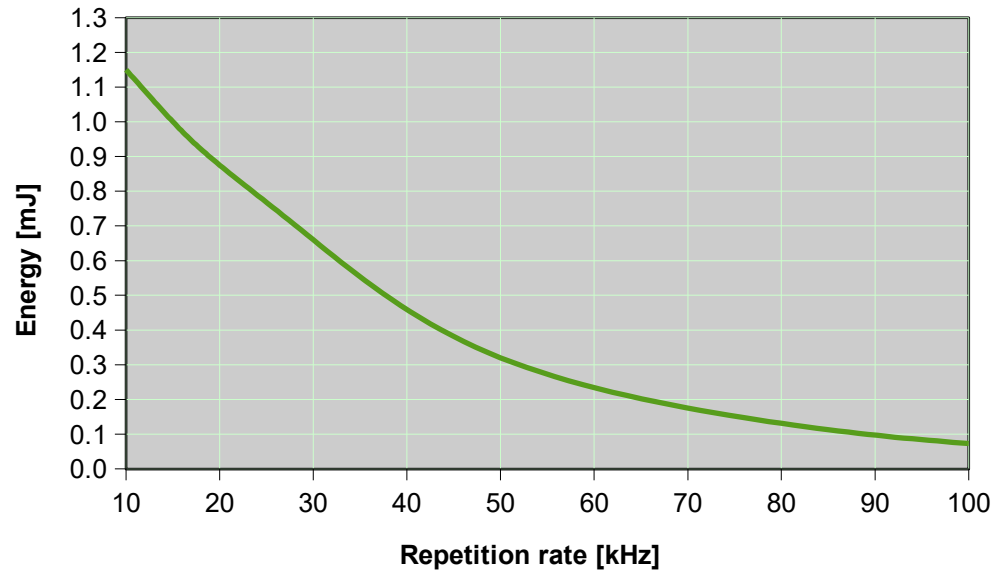
Sol 20W 532nm: Pulse Energy
