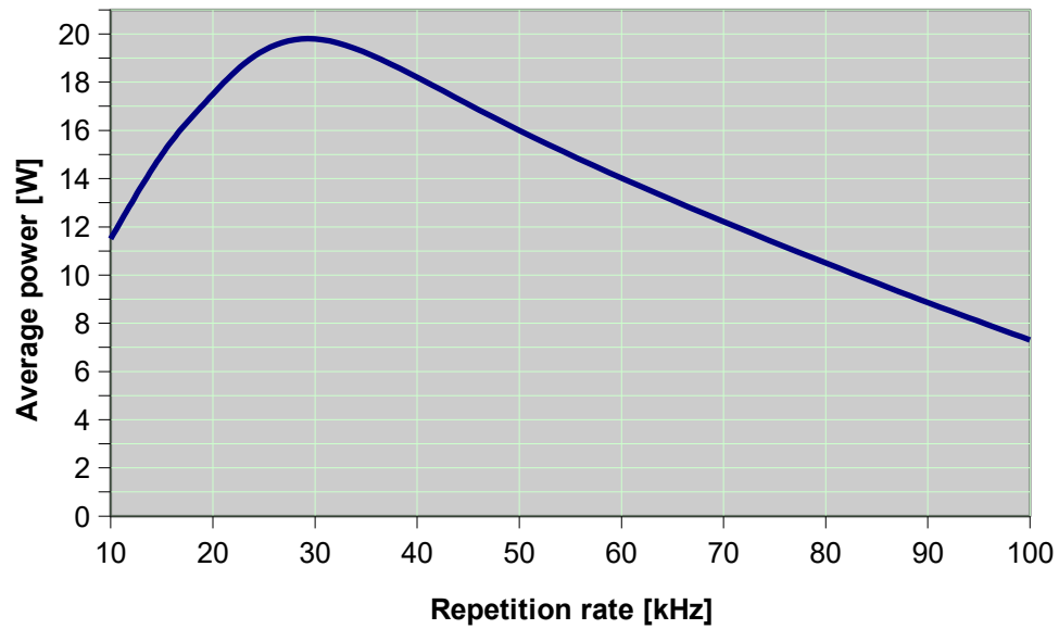
Sol 20W 532nm: Average Power
